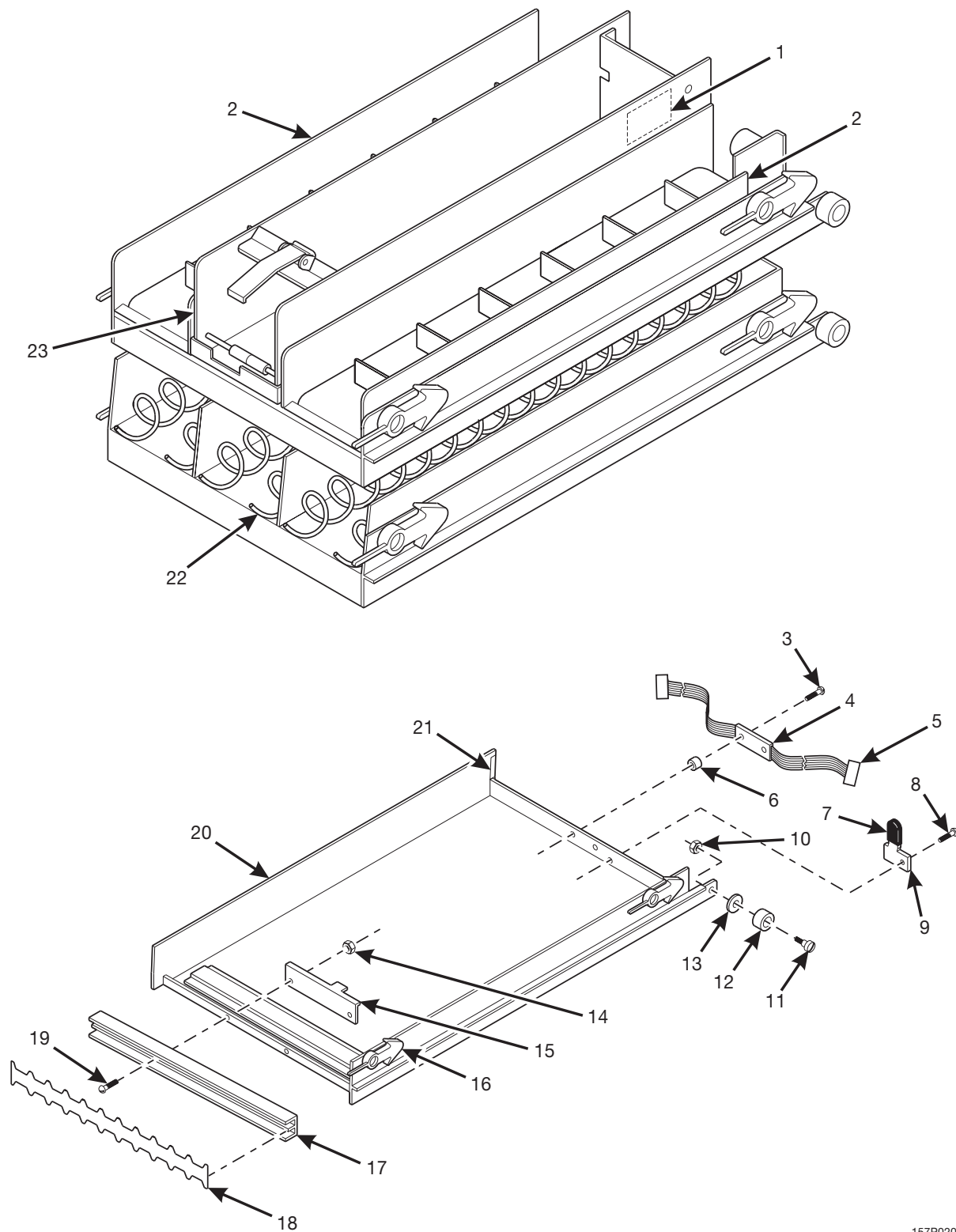
Figure 46. General Tray Assemblies - Refrigerated Food Module
