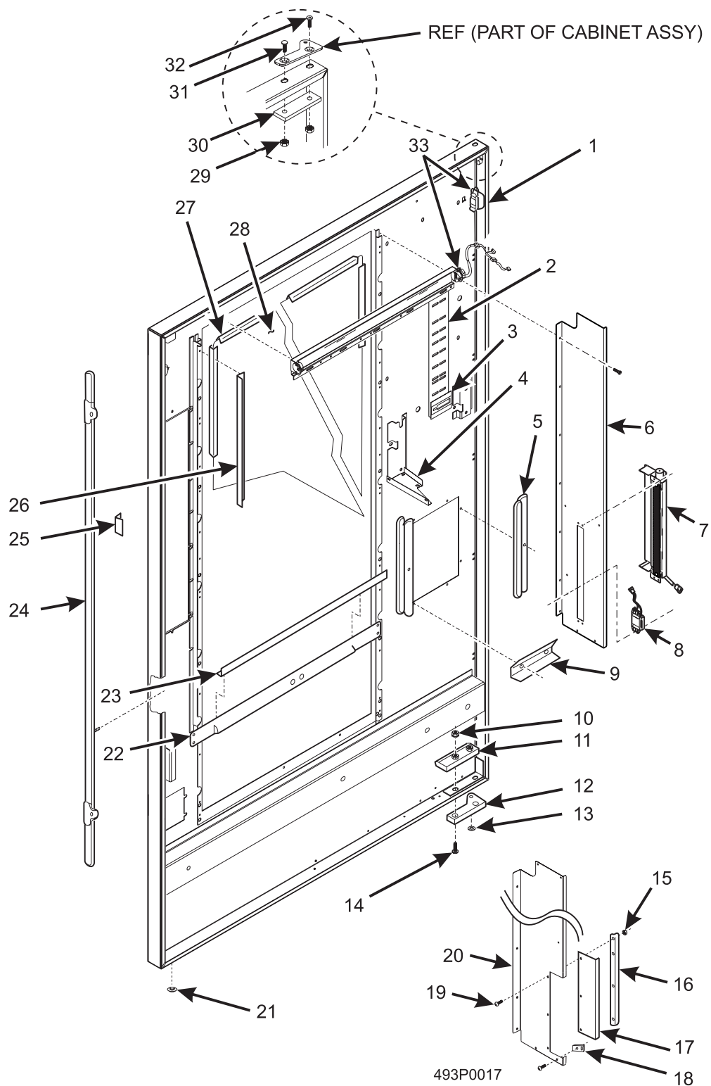
Figure 5. Door Assembly
