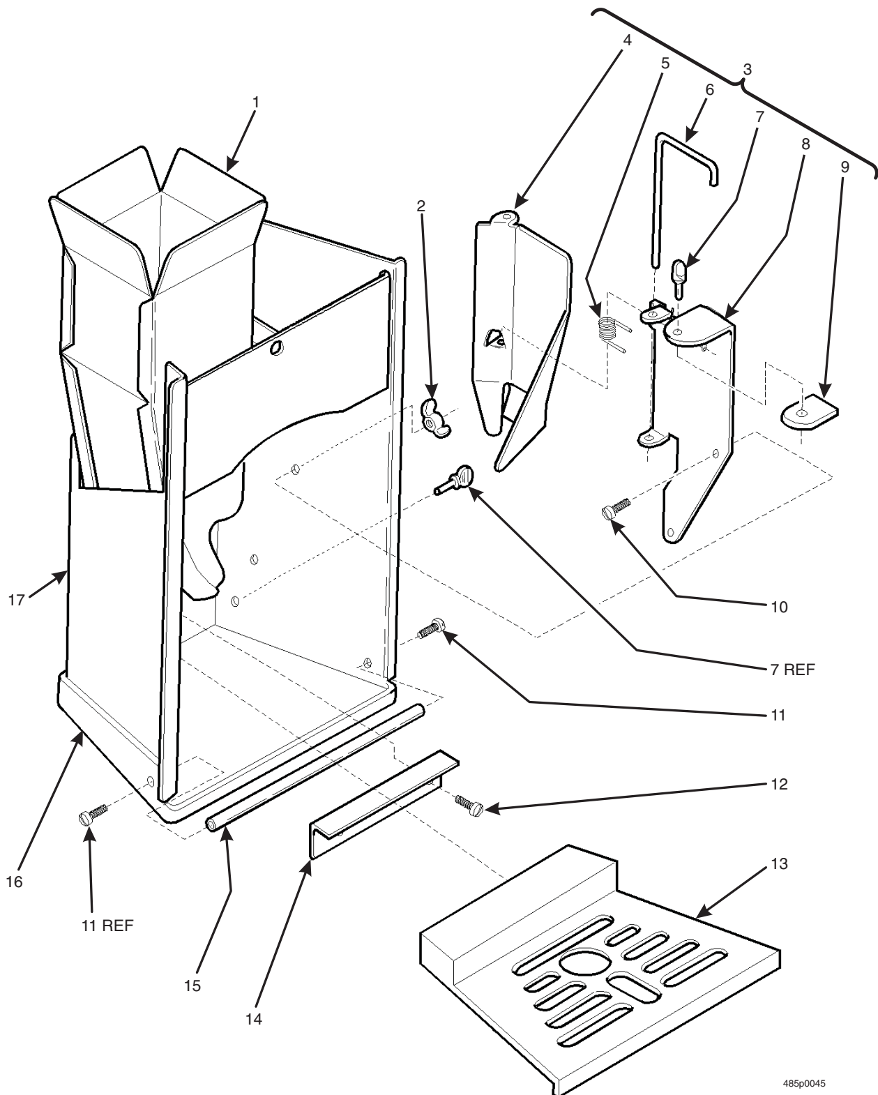
Figure 74. Cup Station Assembly
