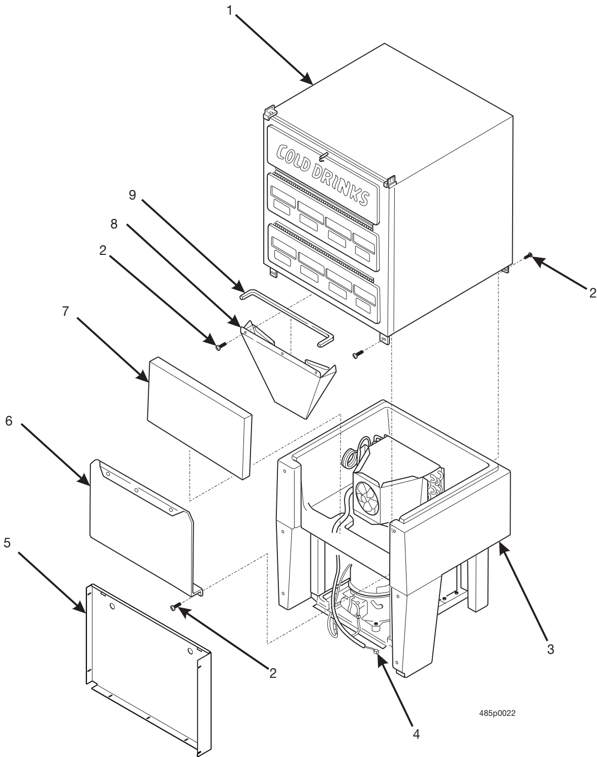
Figure 35. Can and Refrigeration Module
